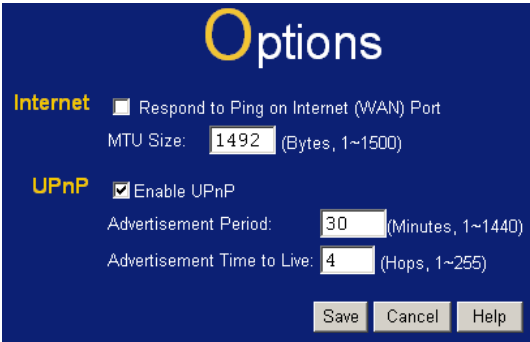
Figure 34: Options Screen
